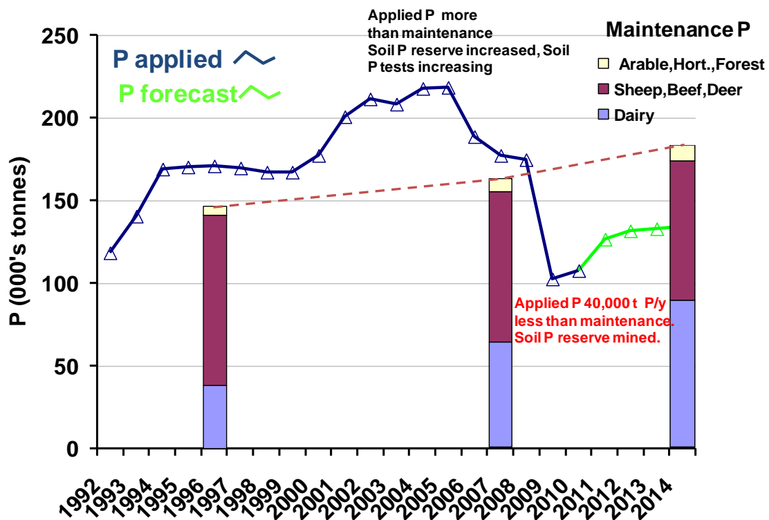
Figure 8. . Quantities of total P applied to pastoral farms (line) and the national maintenance P requirement (columns) calculated from livestock inventories using recommended P replacement rates given in Table 2. (2011-2014 predicted values).
